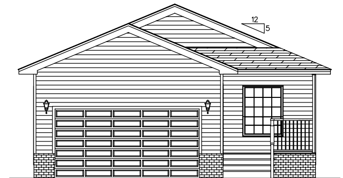
FRONT END ELEVATION
