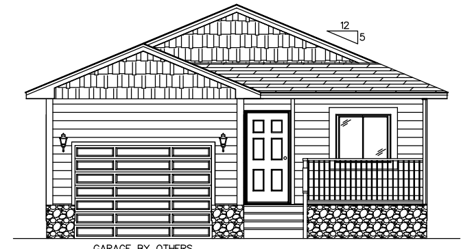
FRONT END ELEVATION
